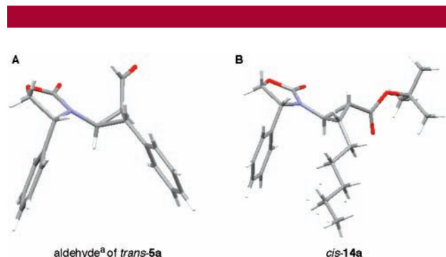
Figure 1. X-ray structures of trans - and cis -amidocyclopropanes. (a) Derived from trans - 5a via Dibal-H [H] (see the Supporting Information).
